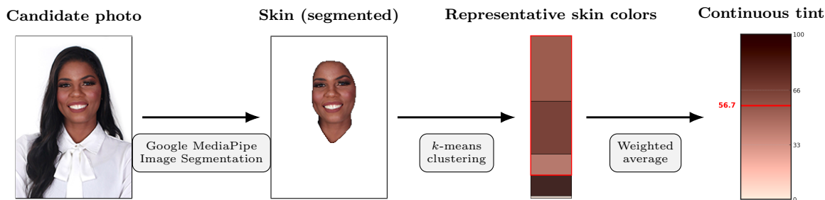
Figure 1: Skin Tone Extraction Pipeline
